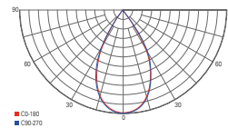
60° wide beam angle with optional 60° lens
