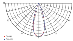
36° standard beam angle with 36° lens [standard]
