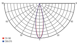
24° narrow beam angle with optional 24° lens
